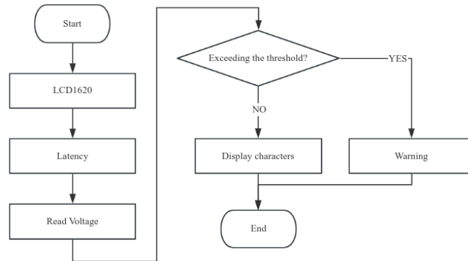
Fig. 10. Show Flowchart
