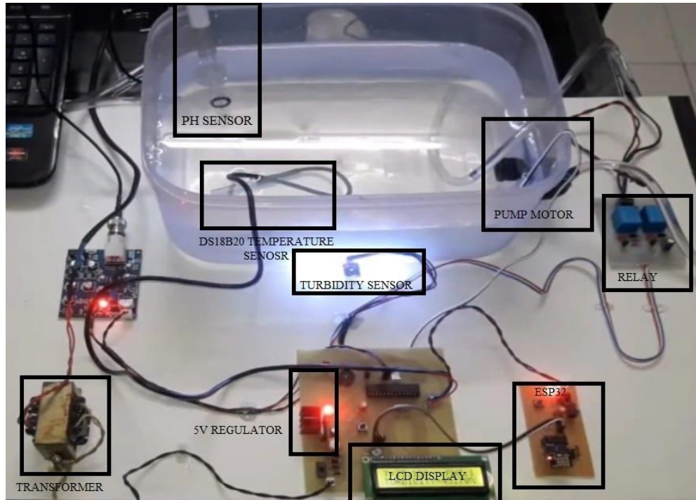
Fig. 9. Prototype model of the proposed model.
