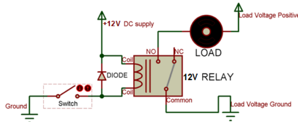
Fig. 7. 12v Relay
