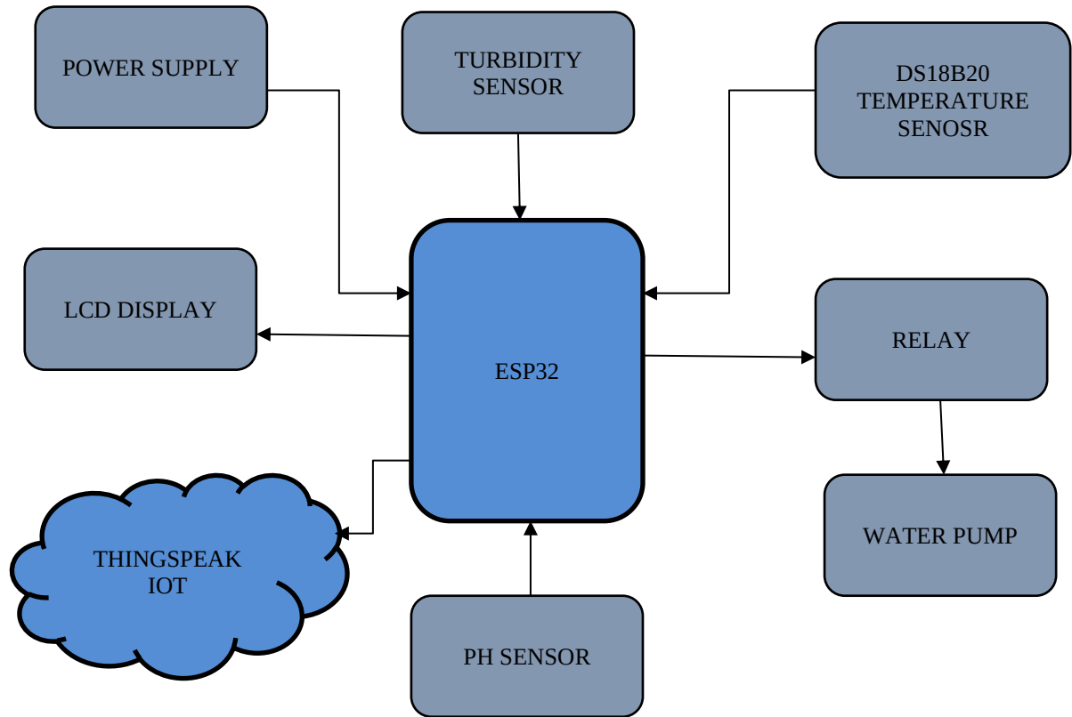
Fig. 1. Block diagram of the proposed Iot-Enabled Smart Aquarium Systems
