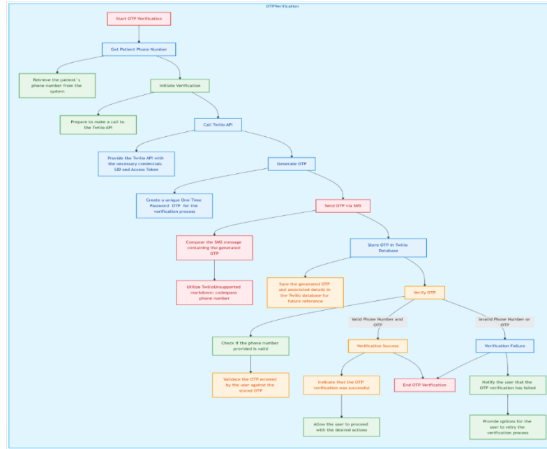
Fig. 8. one time password
