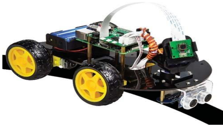
Fig.12. Line following
