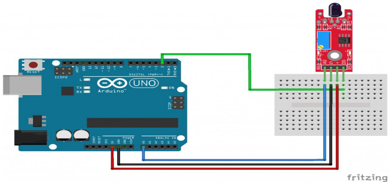
Fig.8. IR flame/fire sensor with Arduino UNO
