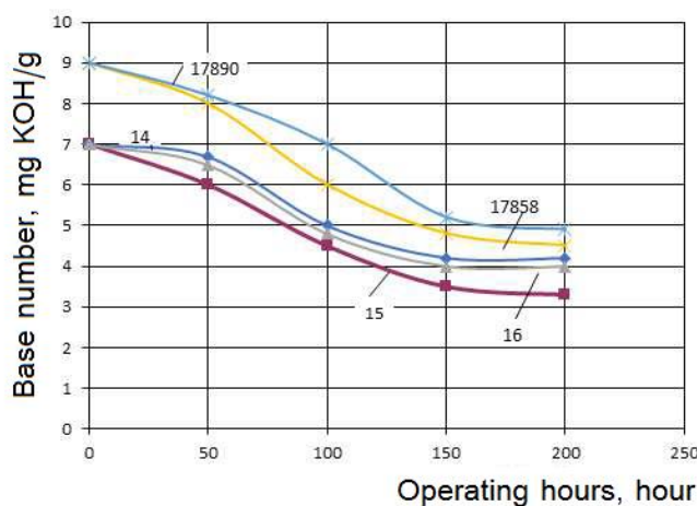
Fig .2. Dependence of changes in the base number content on the operating time of combine engines using M-10G2 and M-10DM engine oils.
