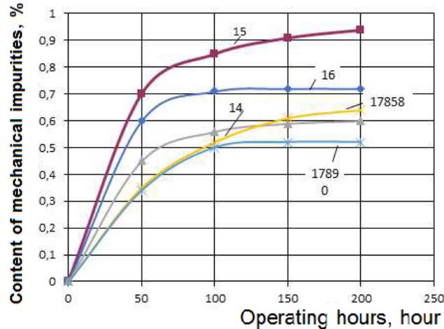
Fig. 3. Change in the content of mechanical impurities
