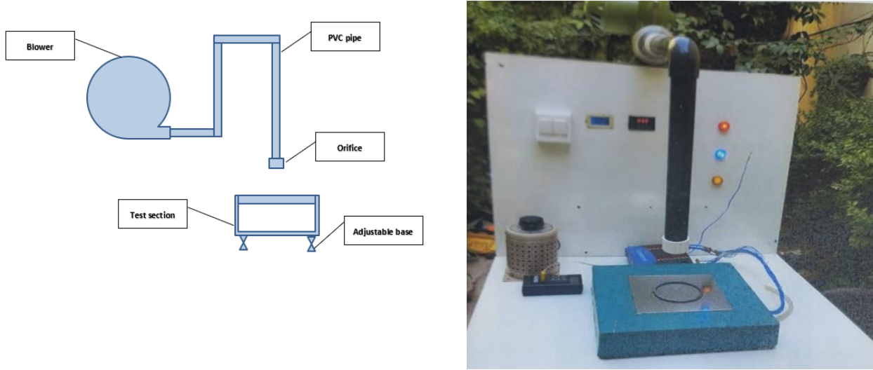
Fig. 2. Schematic and photo of the rig.
