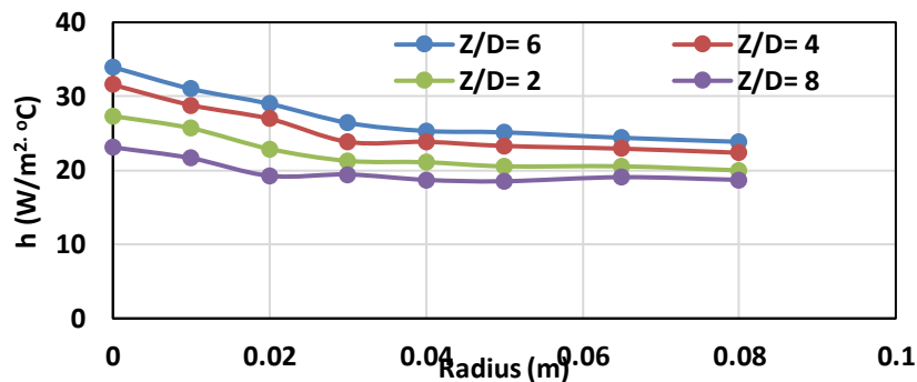
Fig. 4. Effect of Z/D ratio on local heat transfer coefficient ( V=3 m/s, D=10 mm).
