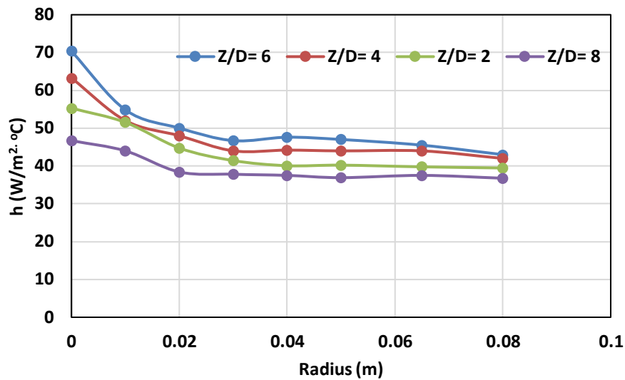
Fig. 5. Effect of Z/D ratio on local heat transfer coefficient ( V=7.2 m/s, D = 10 mm).
