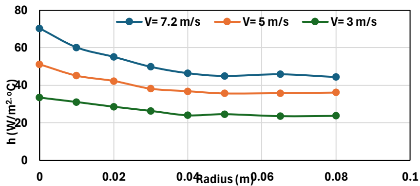
Fig. 7. Effect of velocity on local heat transfer coefficient.
