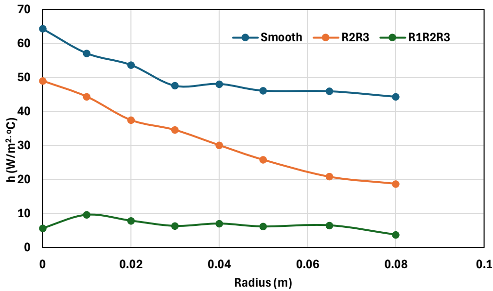
Fig. 10. Effect of rib arrangement on the local heat transfer ( V=7 m/s, Z/D=5 , and D=10 mm)
