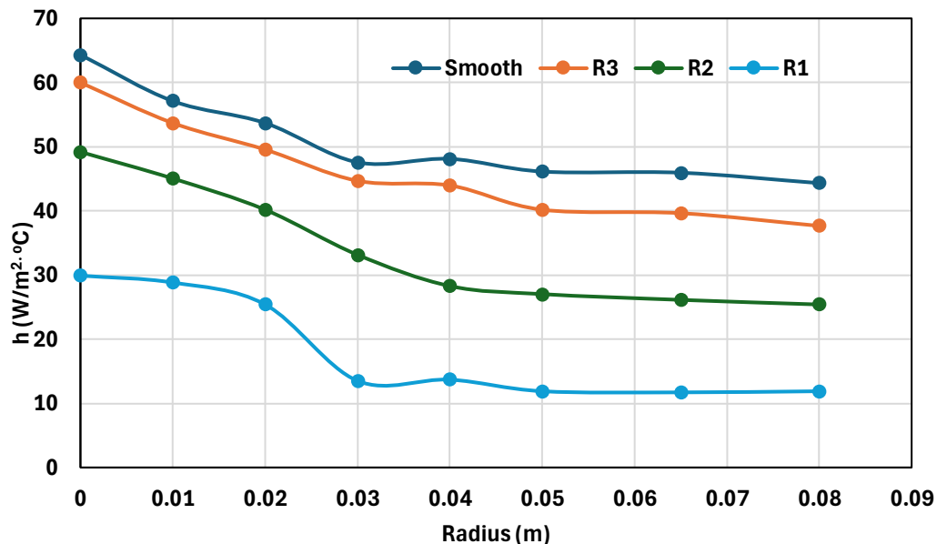
Fig. 9. Effect of rib size on the local heat transfer ( V=7 m/s, Z/D=5 , and D=10 mm)
