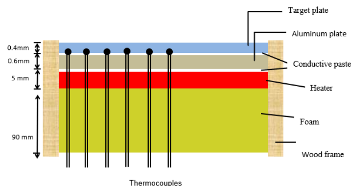
Fig. 1. Section of the test section
