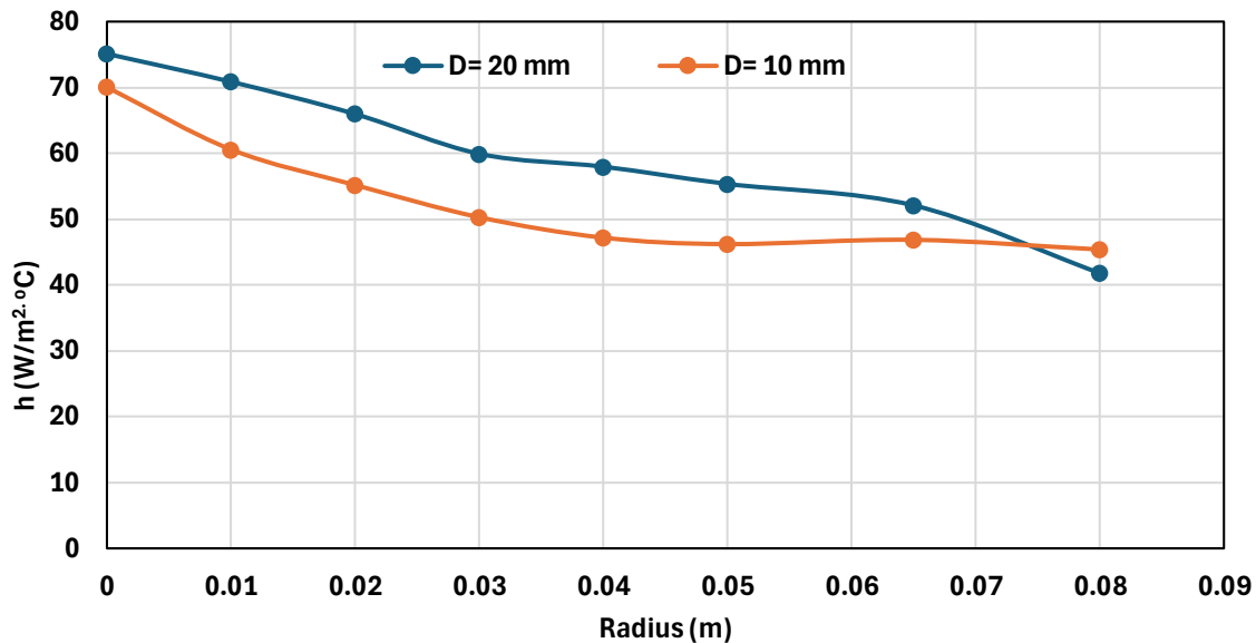
Fig. 8. Effect of diameter on local heat transfer coefficient.
