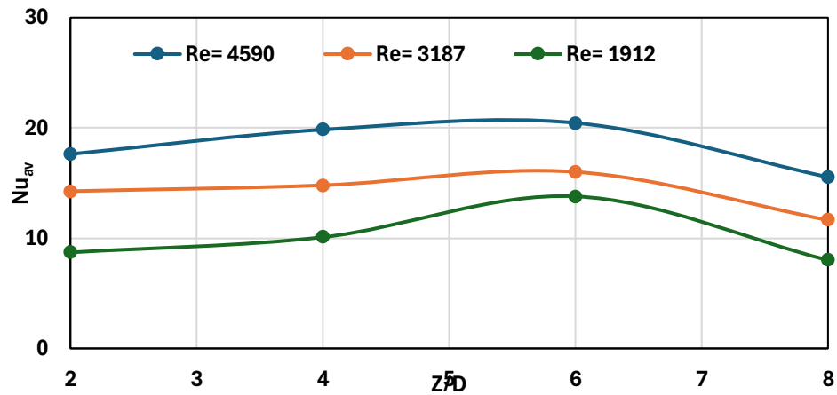
Fig. 6. Variation of Average Nusselt number with Z/D and Reynolds number.
