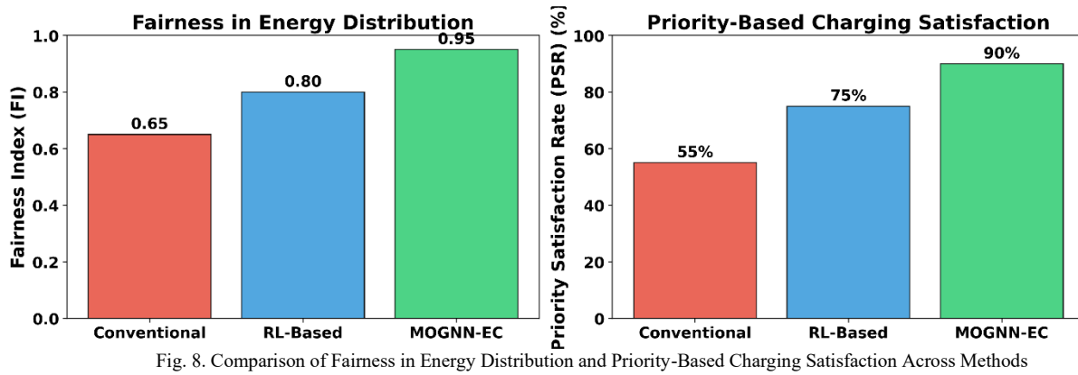
Fig. 8. Comparison of Fairness in Energy Distribution and Priority-Based Charging Satisfaction Across Methods
