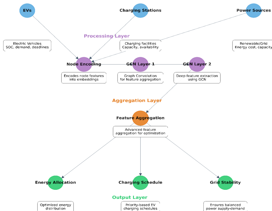
Fig. 2. Architecture of the MOGNN-EC Model
