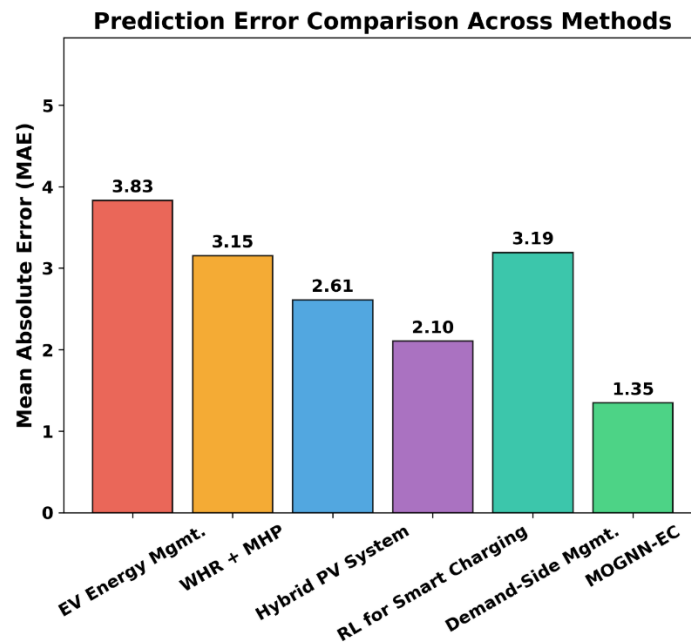
Fig. 9. Prediction Error Comparison Across Methods Using Mean Absolute Error (MAE)
