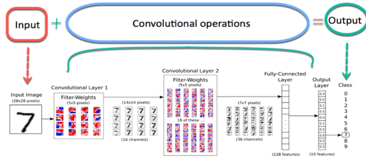
Fig.3. Convolutional Operations
