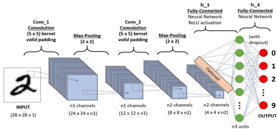
Fig.6. Convolutional Neural Network (CNN) model
