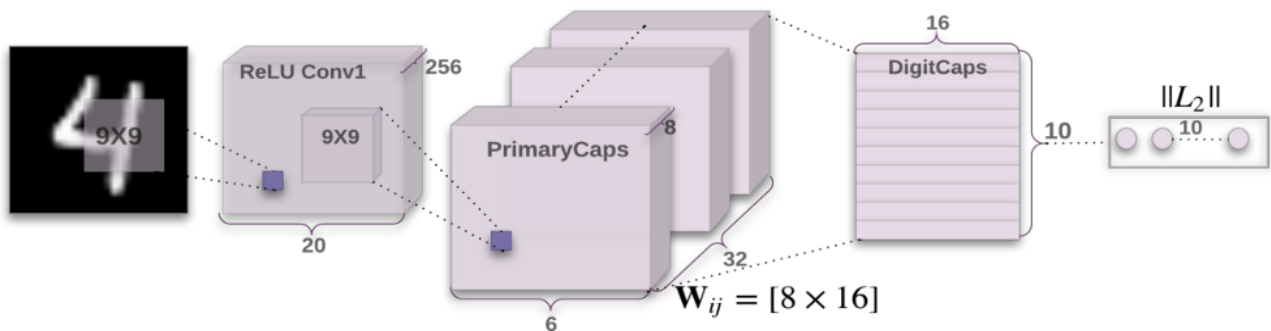
Fig .2. Typical Caps Net architecture [1].
