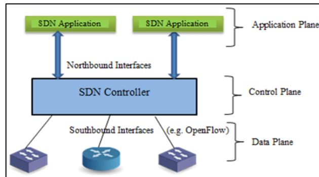
Fig.3. SDN architecture
