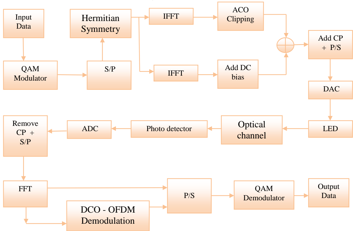
Fig. 4. LACO-OFDM.
