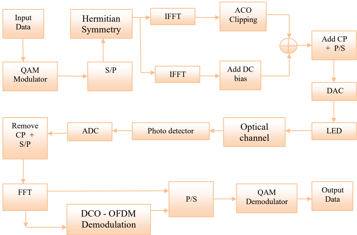
Fig. 4. LACO-OFDM.
