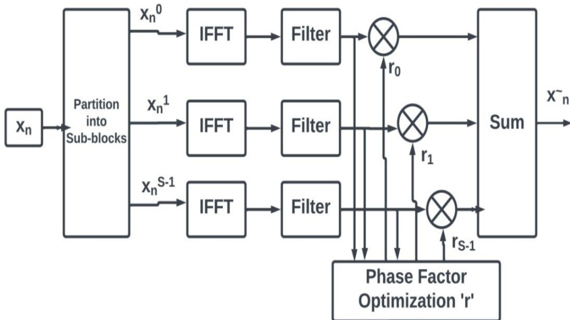
Fig. 6. PTS digram
