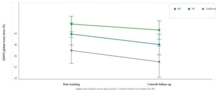
Fig. 5. OSATS global performance scores immediately post-training and after one month for AR, VR, and Traditional groups (n = 10 each)
