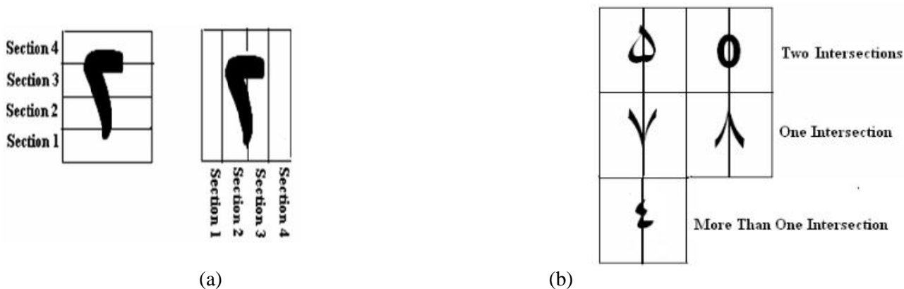
Fig.12. a) Divide picture to four horizontal and four vertical section, b) Count the number of intersections along middle vertical ray [19]
