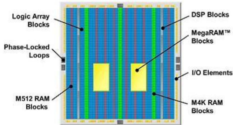
Fig.9. Altera FPGA Structure
