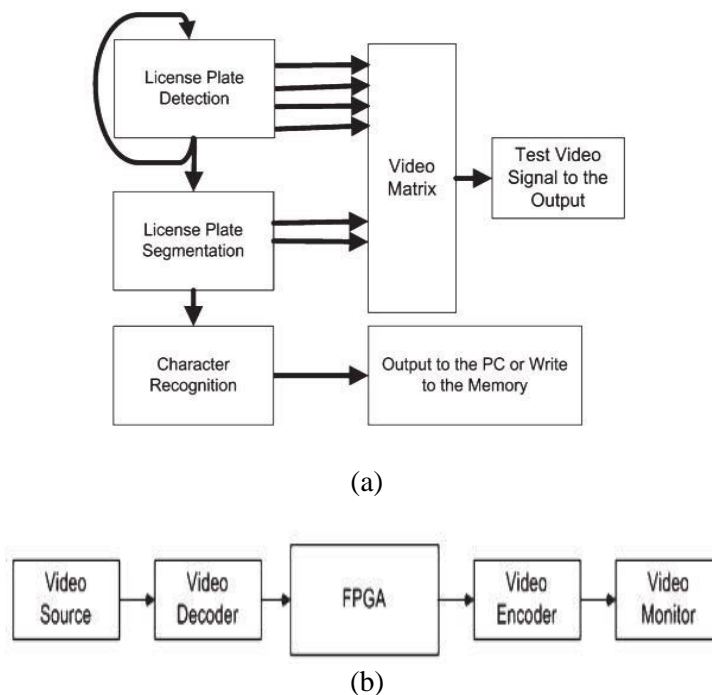
Fig.15. a) Embedded LPR system block diagram, b) Hardware block diagram [23]
