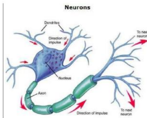
Fig.6. Neuron Components
