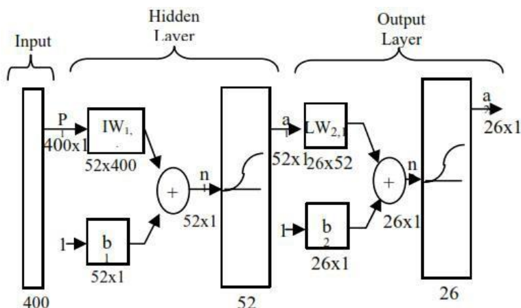
Fig.4. Neural Network Architecture [7]
