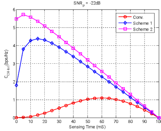
Fig.2. CR-IoT Throughput versus Sensing Time
