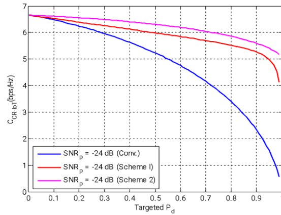
Fig.3. CR-IoT Throughput versus targeted Probability of detection
