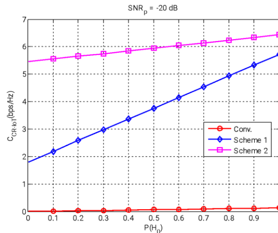
Fig.6. CR-IoT Throughput versus Probability of PU Absence from licensed channel
