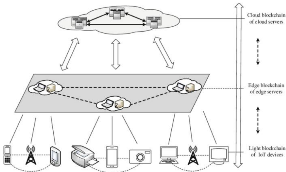
Fig.1. Overall framework
